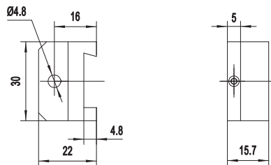
APFP-GH GRIN Lens Mount (Fiber Diameter < 4.8mm)
