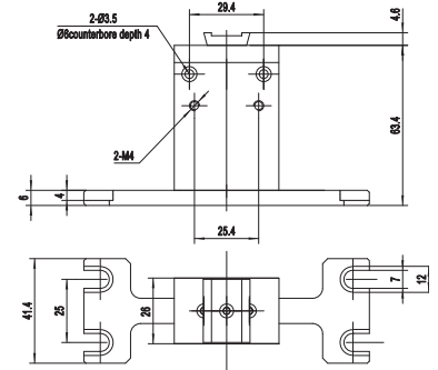
APFP-TS Fixed Platform, Narrow Profile T-Stand
