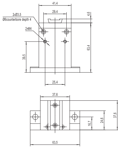
APFP-US Fixed Platform, Universal Stand
